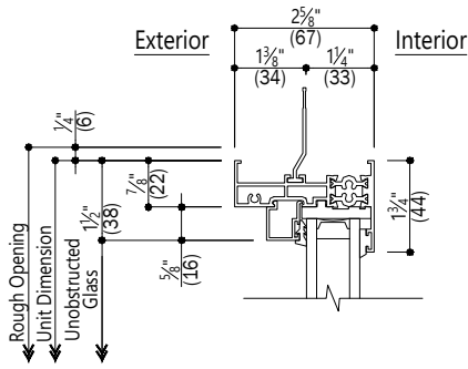
A Head 2 Fixed
