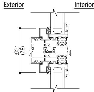
D Horizontal Join 2 Fixed/Fixed
