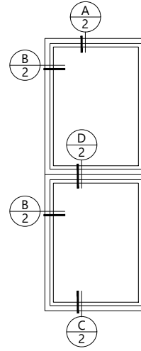
Fixed Over Fixed Non-integral Join
