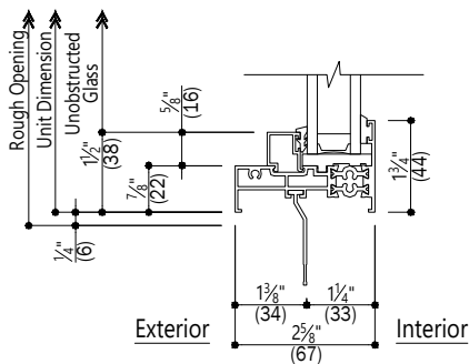
C Sill 2 Fixed
