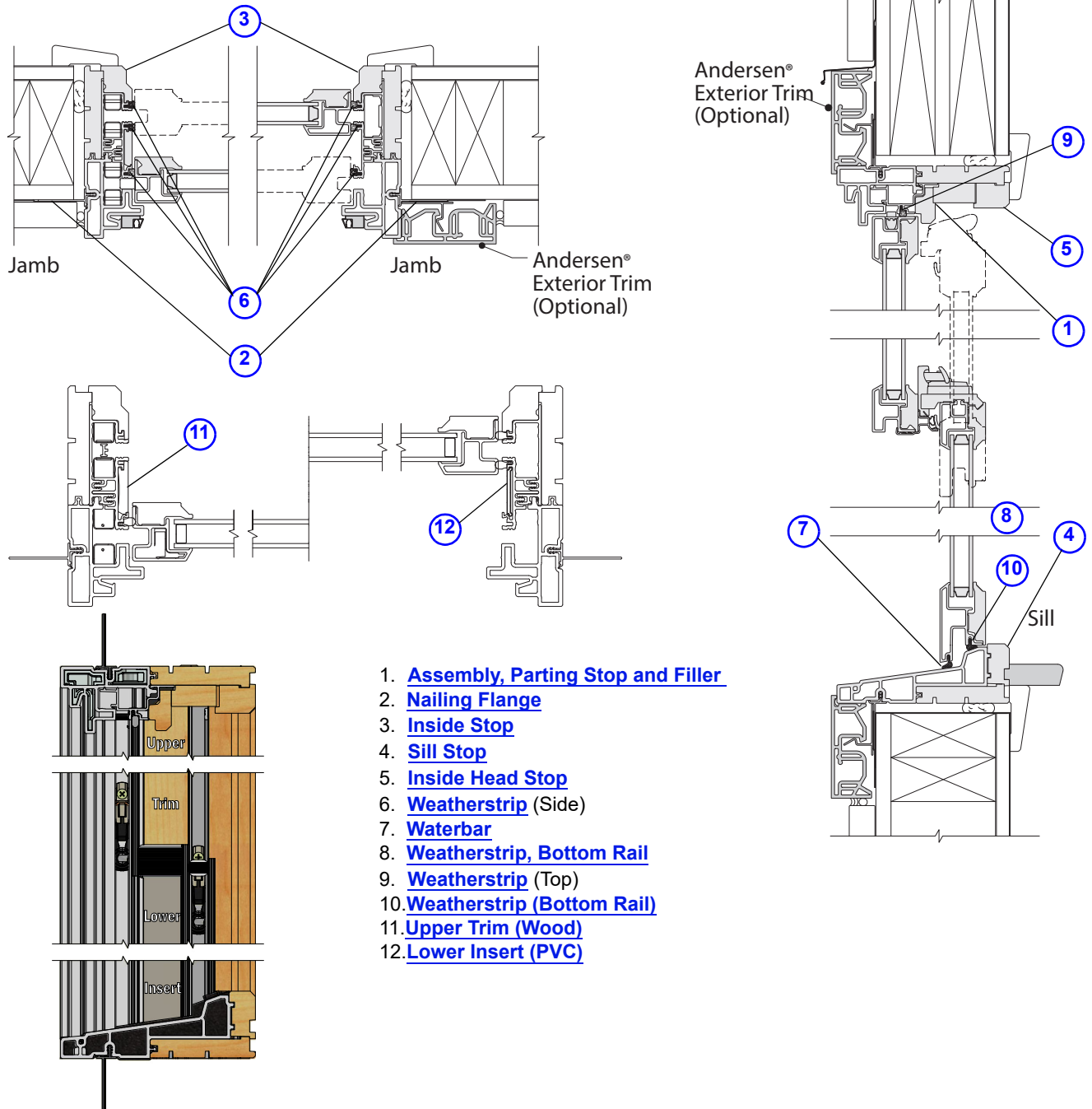
A-Series Double-Hung Windows Frame Assembly
