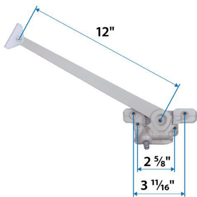
Straight Arm Operator with Screws / 12"
