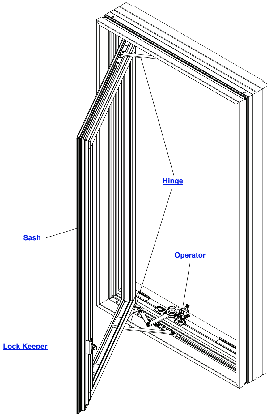
Manufactured 2008 to Present A-Series Casement Window Unit Parts
