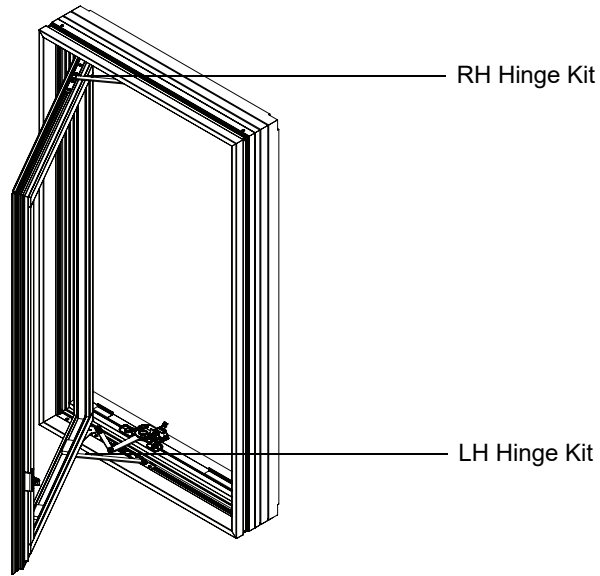
Left-Hand Unit Shown
