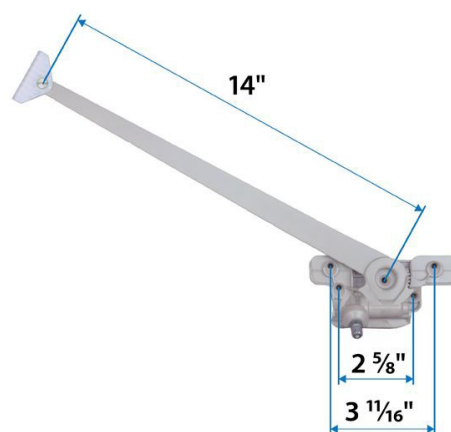
Straight Arm Operator with Screws / 14"
