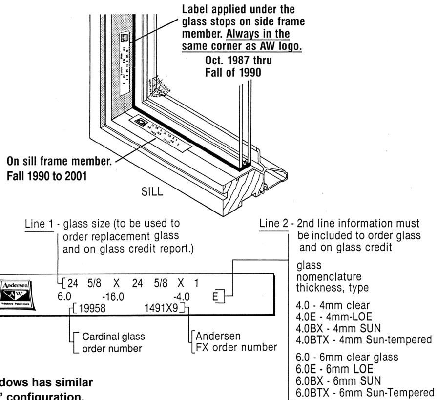
Arch Glass Dimension Label
