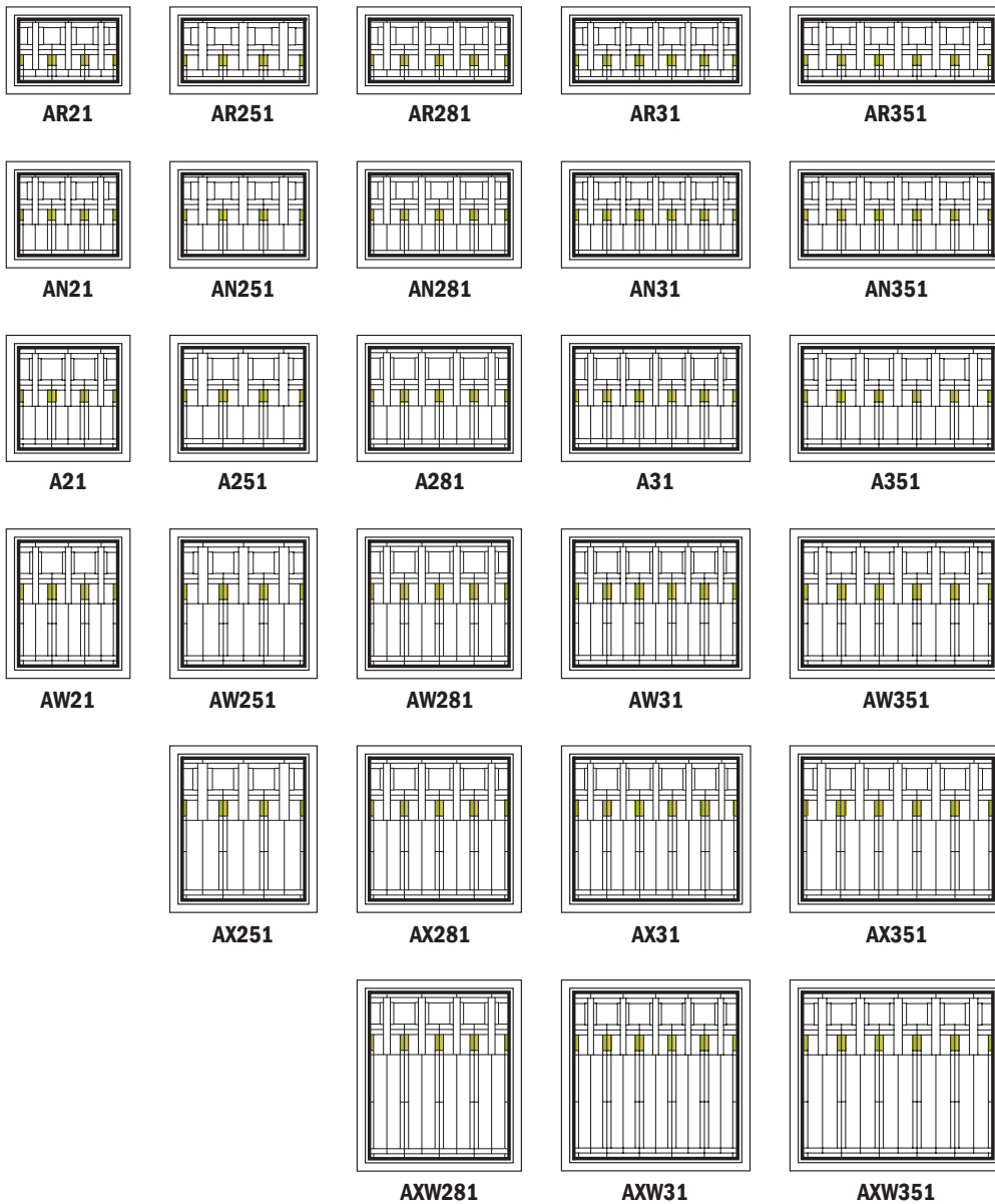
Colonnade Panels for Awning Windows
