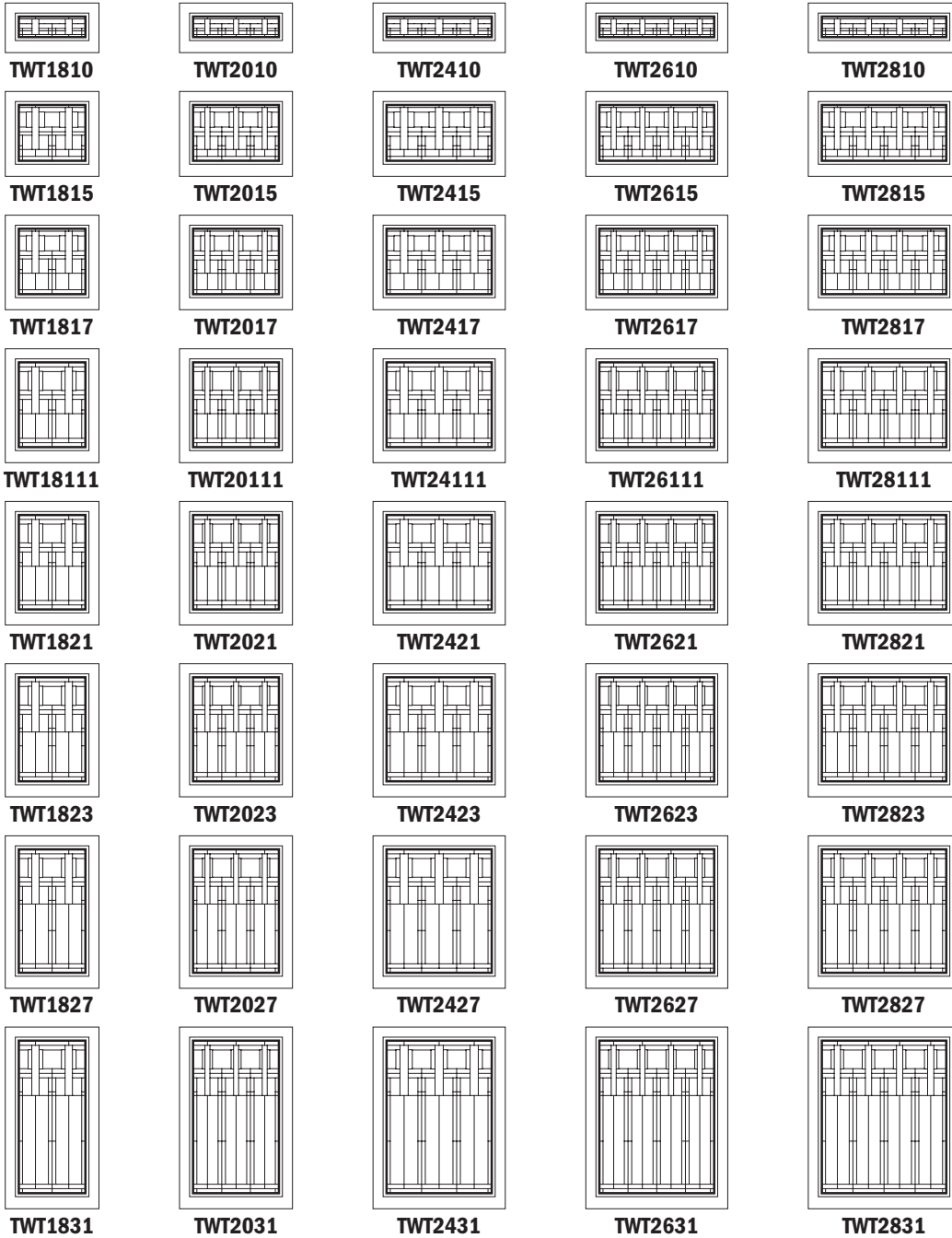
Colonnade Panels for Double Hung Picture, Sidelights, & Transom Windows
