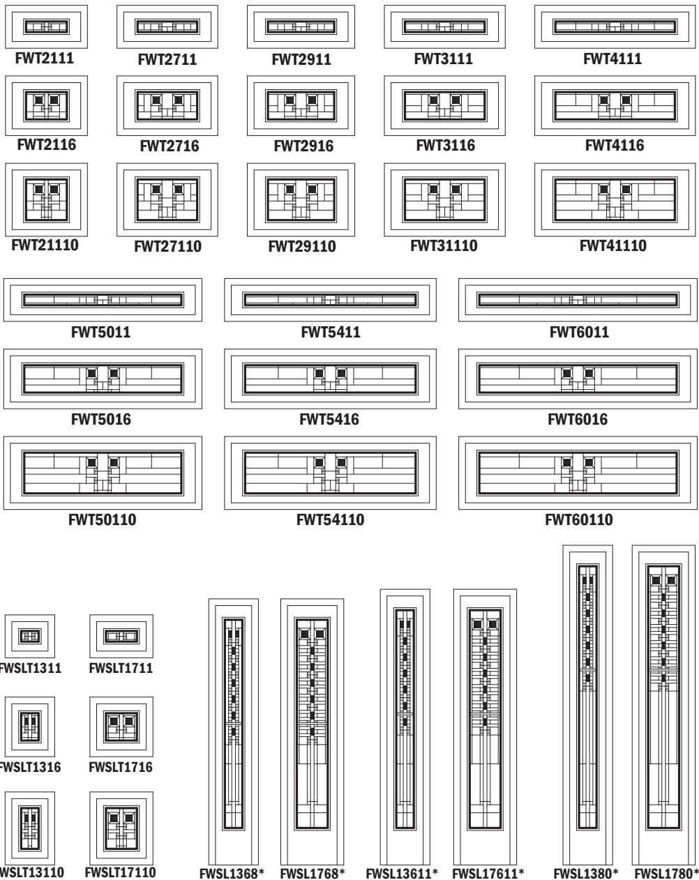
Prairie Rhythm Panels for Frenchwood® Doors Sidelights and Transoms
