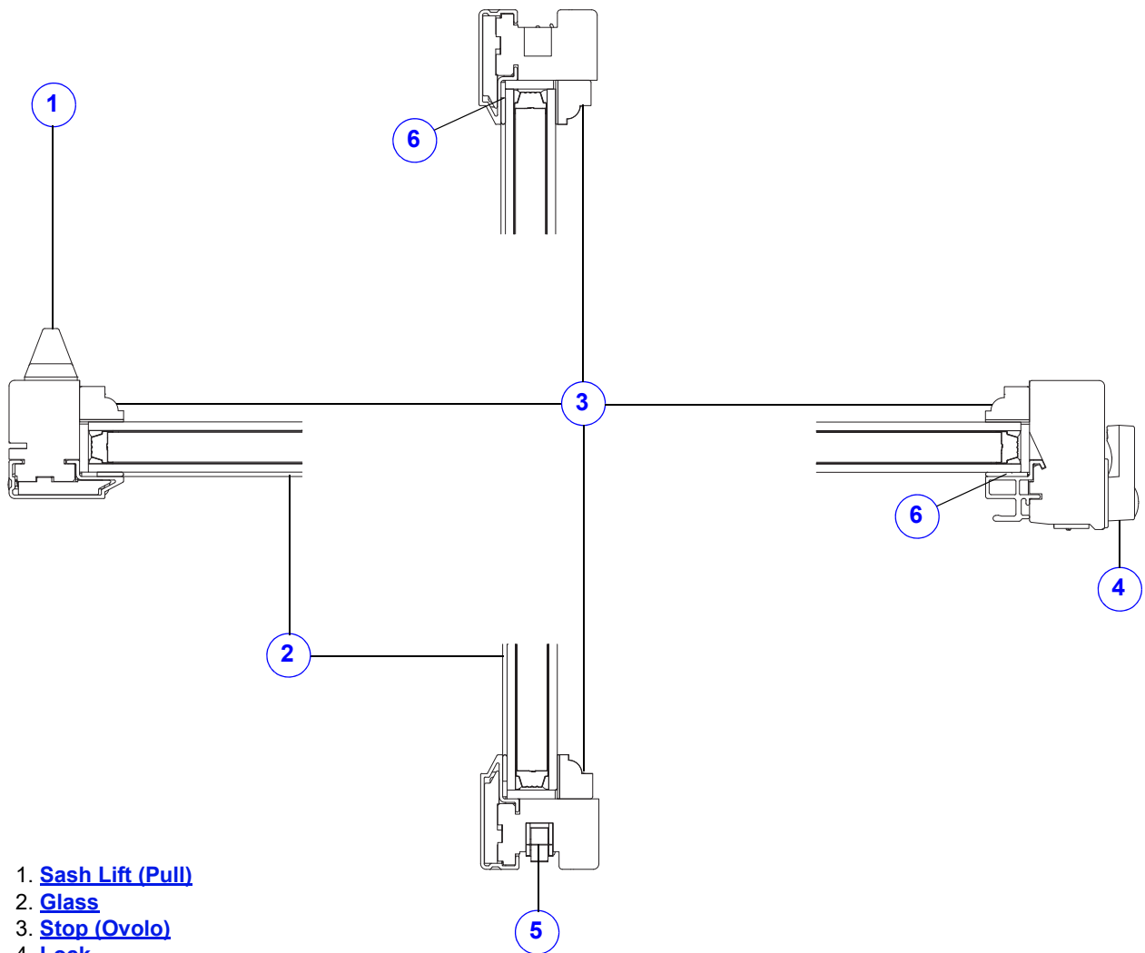
E-Series Gliding Window Sash - Operating
