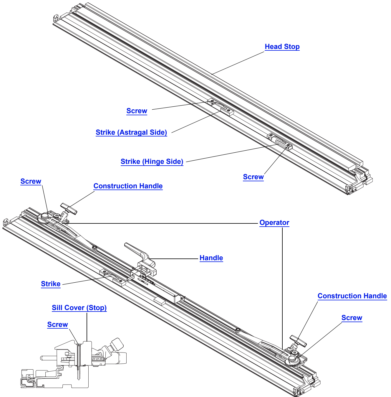
French Casement Frame (Head and Sill) Assembly
