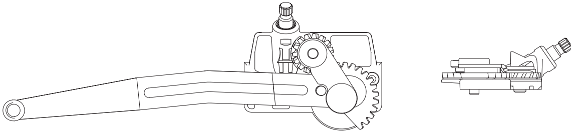
French Casement Operator
