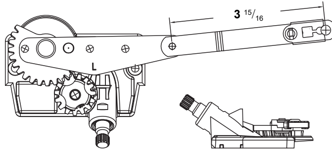
Casement Operator
