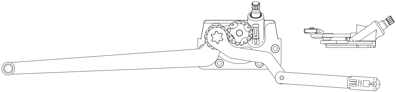
Casement Operator
