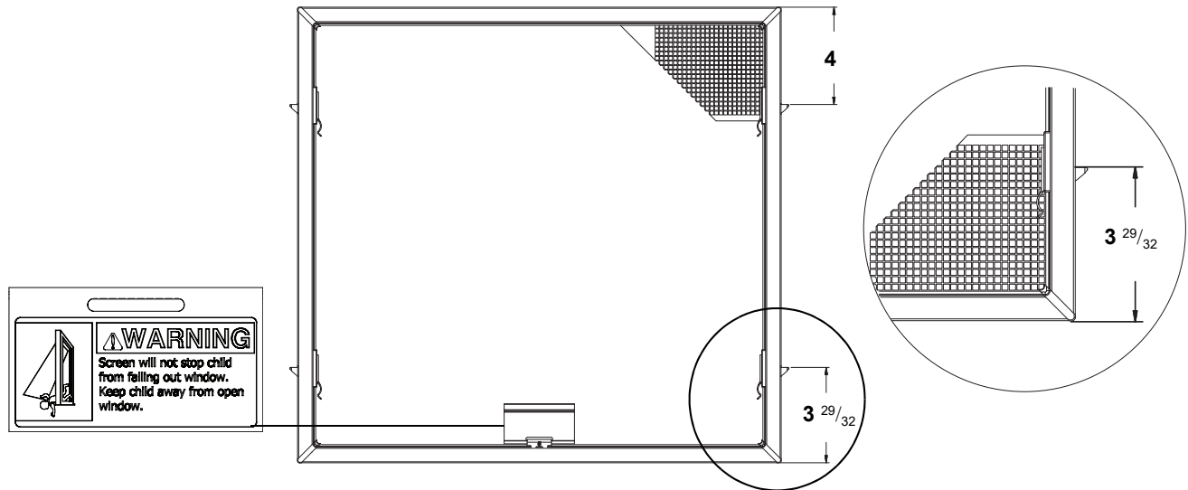
Tilt-Wash Monumental Half Insect Screen
