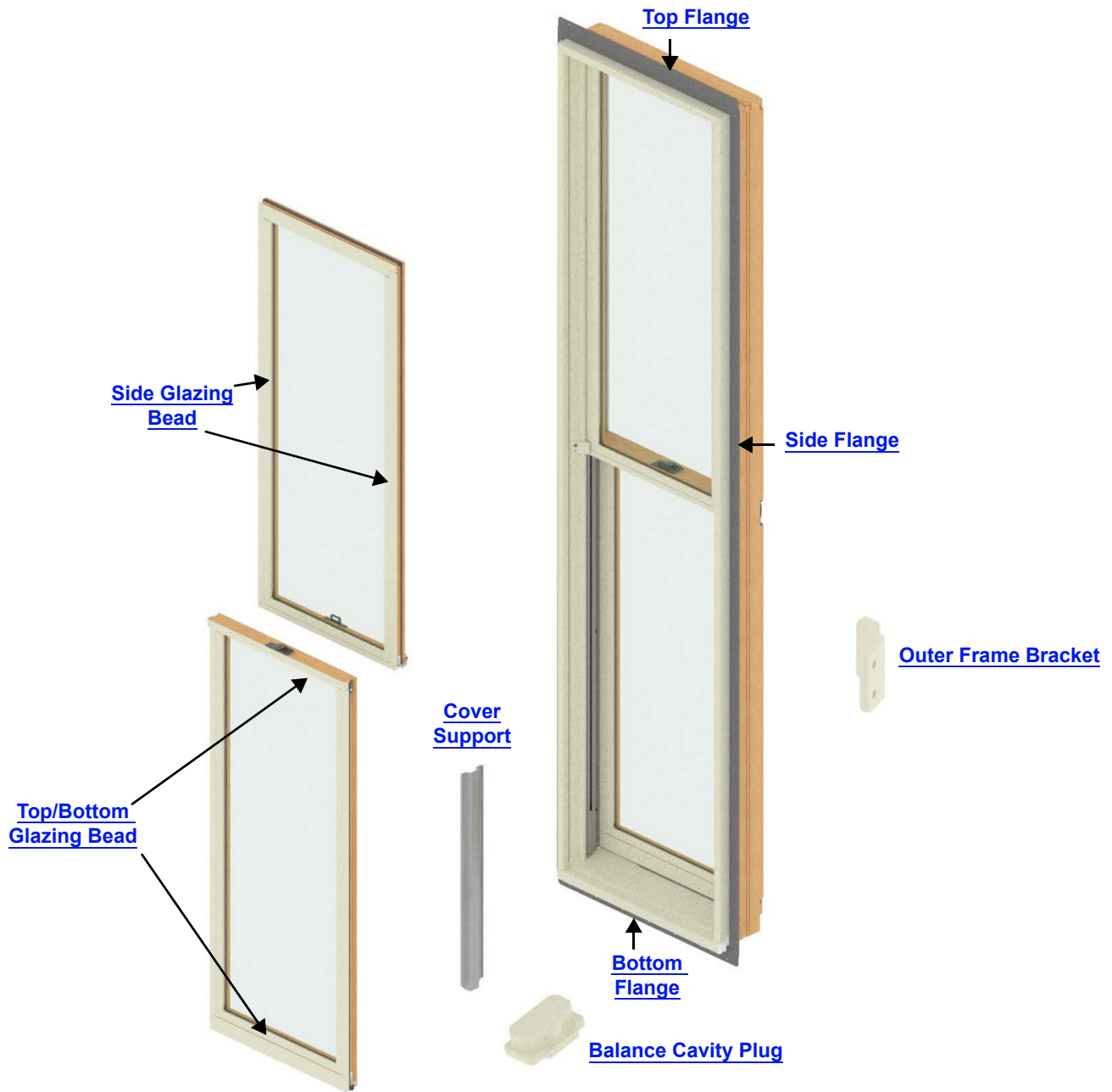
Tilt-Wash Monumental Window Unit Parts
