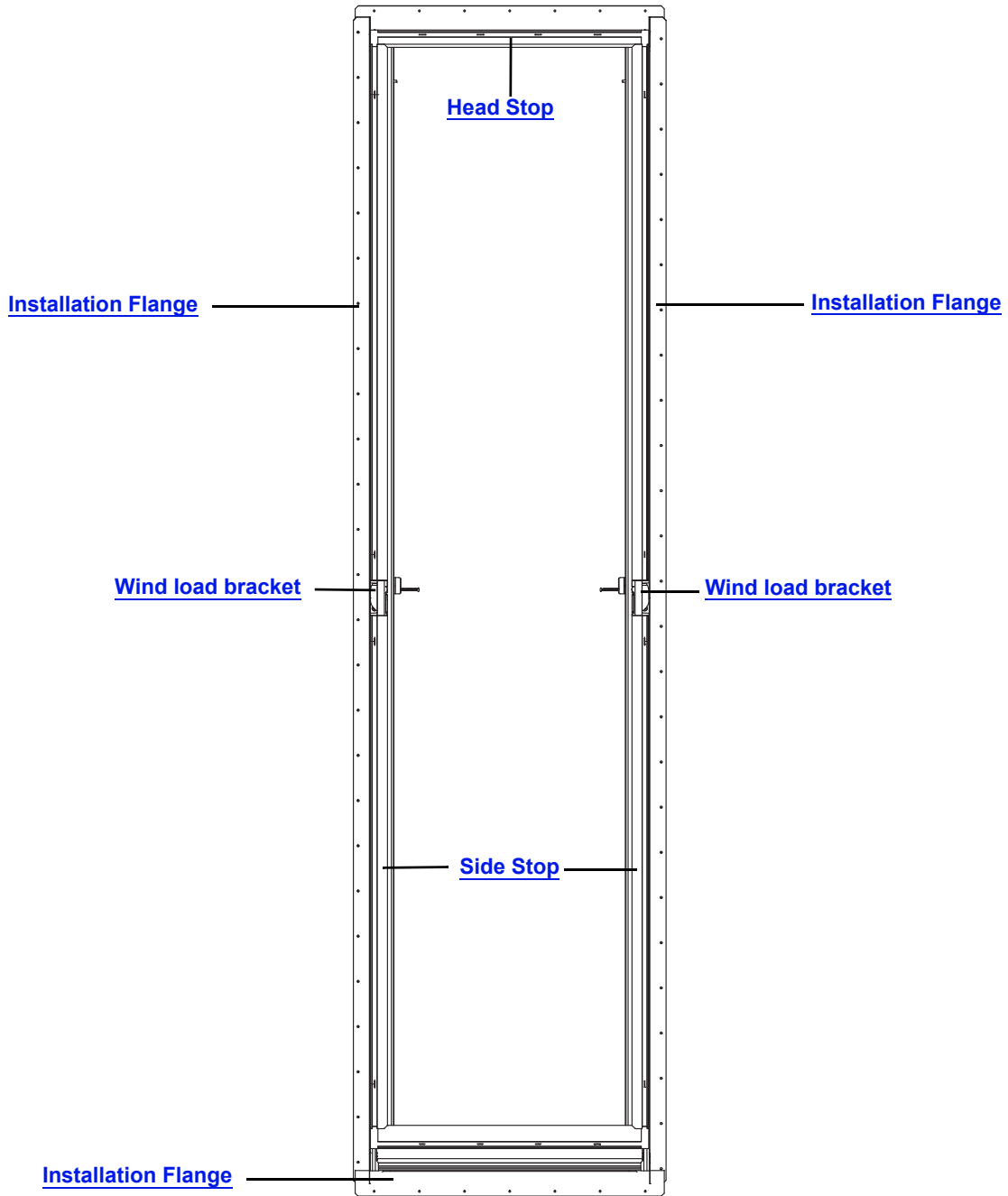
Tilt-Wash Monumental Frame Assembly
