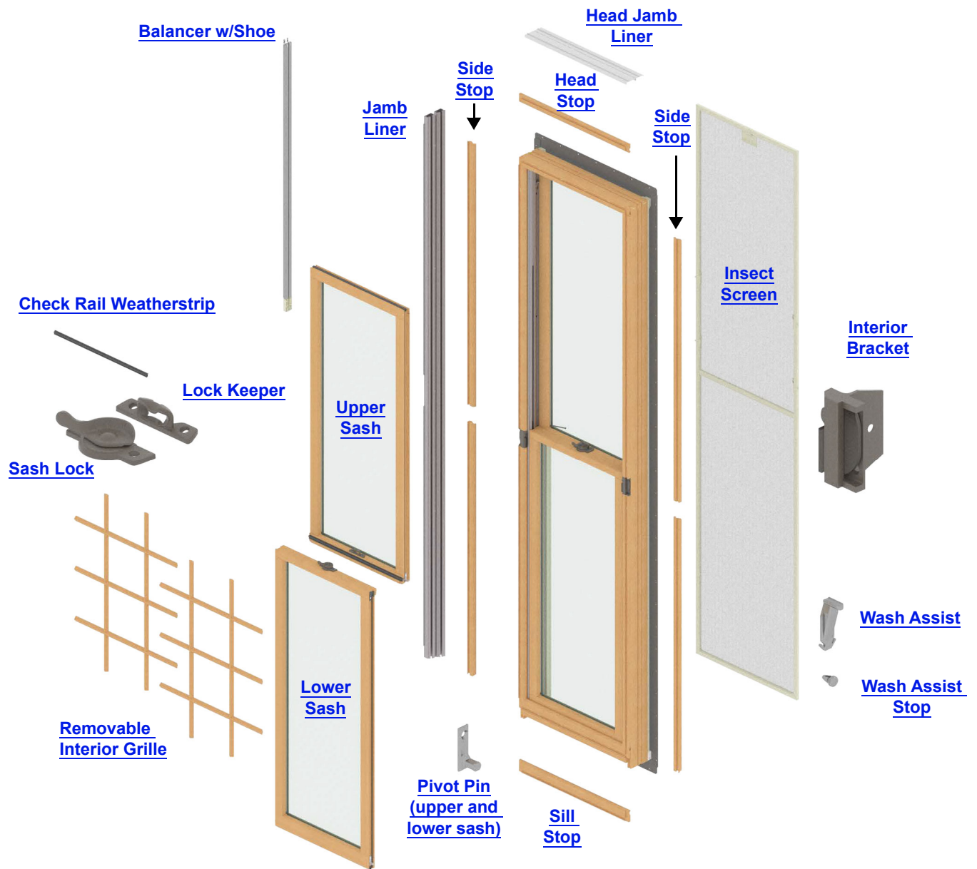
Tilt-Wash Monumental Window Unit Parts
