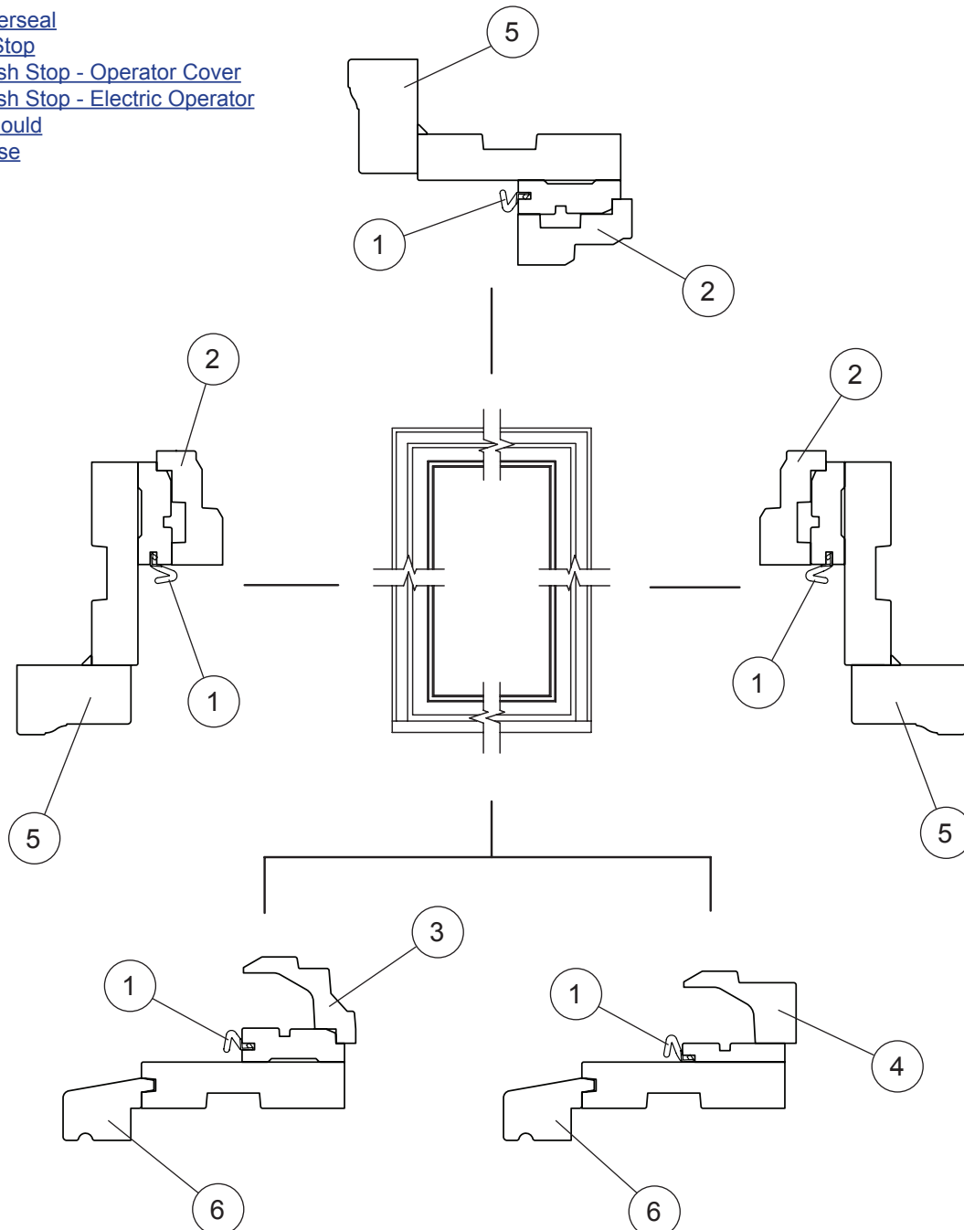
Complementary Wood Awning Windows - Wood Frame
