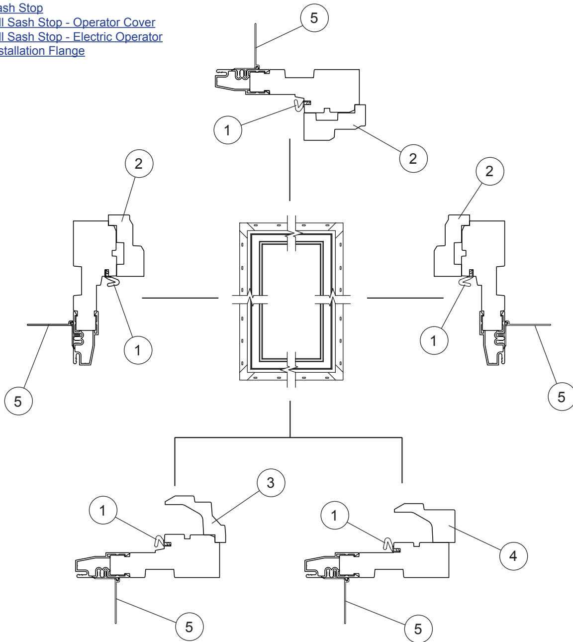
Complementary Clad Awning Windows - Clad Frame
