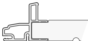
Standard Cladding - PF1904
