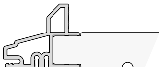
Standard Cladding - PF1200
