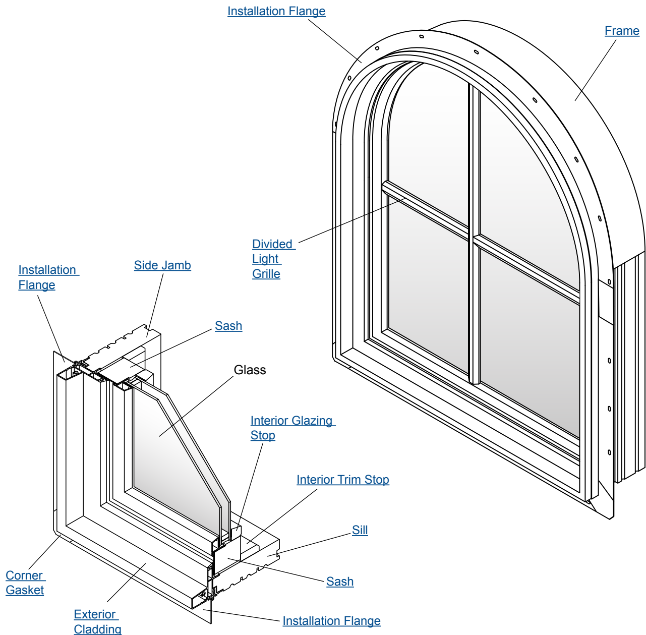
Andersen® Complementary Clad Specialty Fixed Window Unit Parts - Sash Glazed Window
