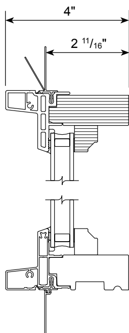
Curved Jamb
