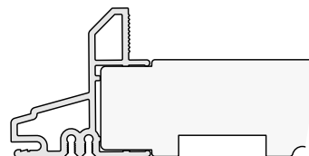
Thick Frame Cladding - PF1301
