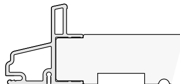
Thick Frame Cladding - PF1905
