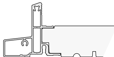
Thick Frame Cladding - PF2146
