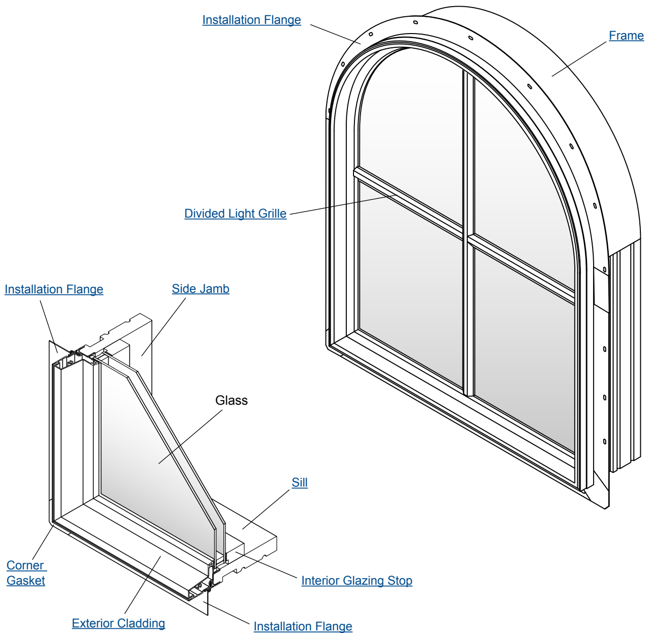
Andersen® Complementary Clad Specialty Fixed Window Unit Parts - Standard Window
