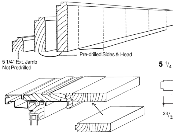
Double-Hung Picture and Sidelight Extension Jamba
