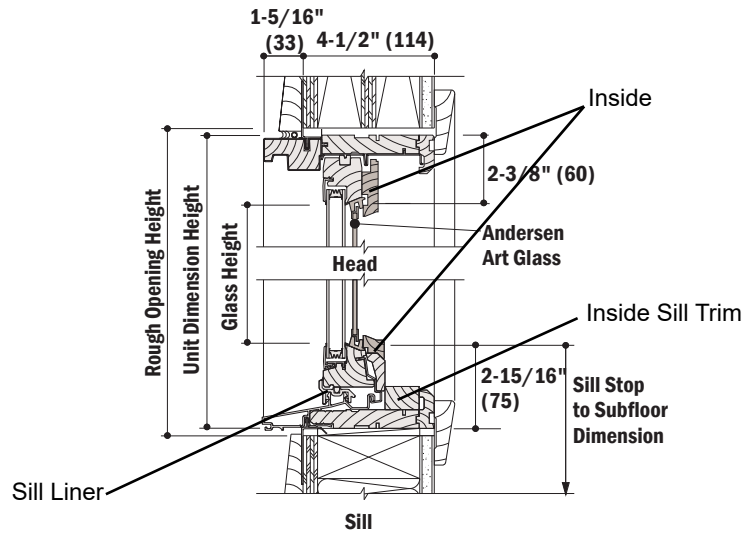
Vertical Section
