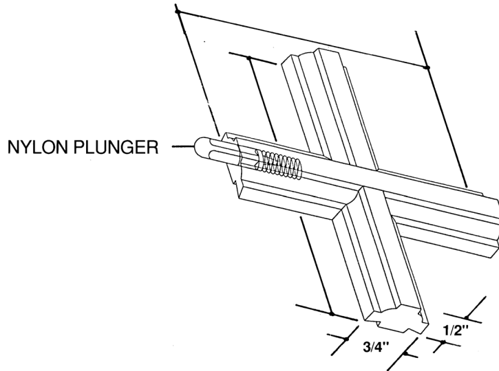
Double-Hung (DH) Interior Wood Grilles - Colonial / 3/4" Wood
