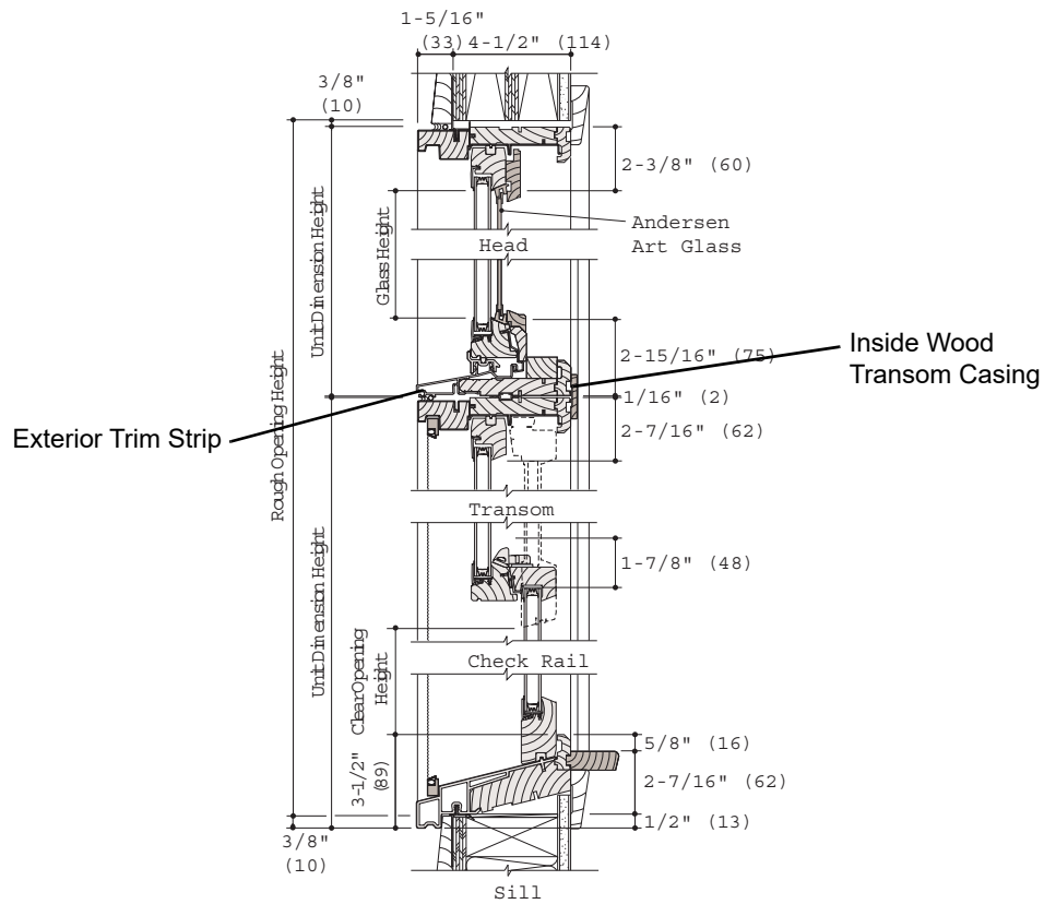
Double-Hung (DH) Transom Window Narrow Mullion
