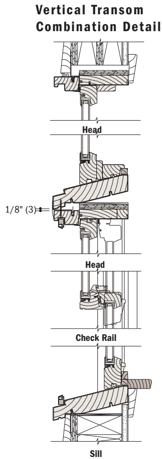
Perma-Shield® Narroline® Transom Joining
