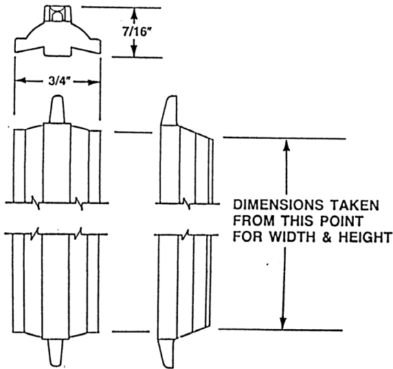
Perma-Shield® Narroline® Transom Window Interior Grilles - 3/4" Polycarbonate
