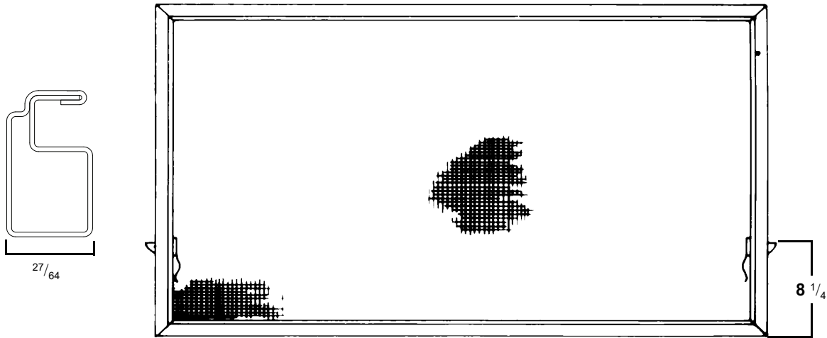
Manufactured July 1994 to 2012 Perma-Shield® Narroline® Combination Unit Insect Screen
