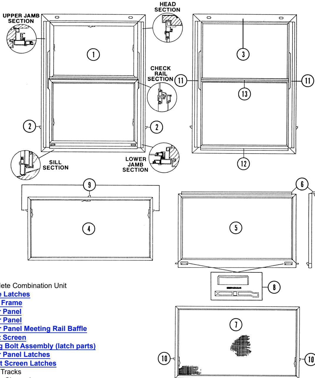
Perma-Shield® Narroline® Combination Units
