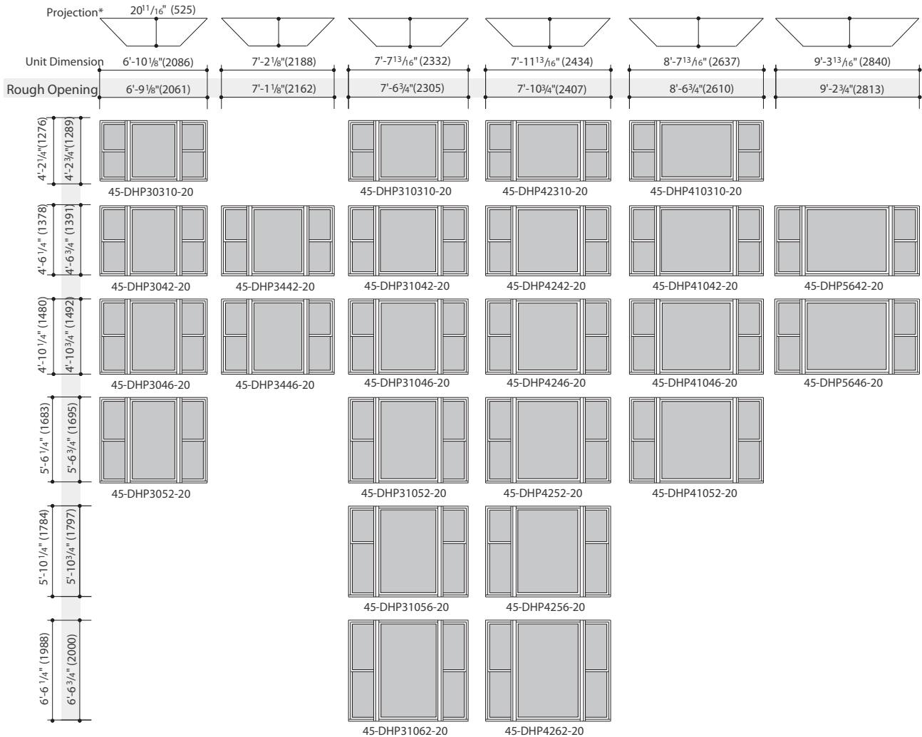
Perma-Shield® Narroline® 45° Angle Bay Window Unit Sizes
