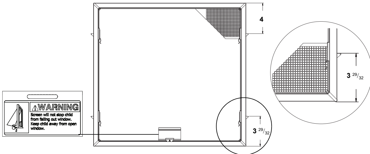
Tilt-Wash (DC) and Tilt-Wash II (TW) Half Insect Screen
