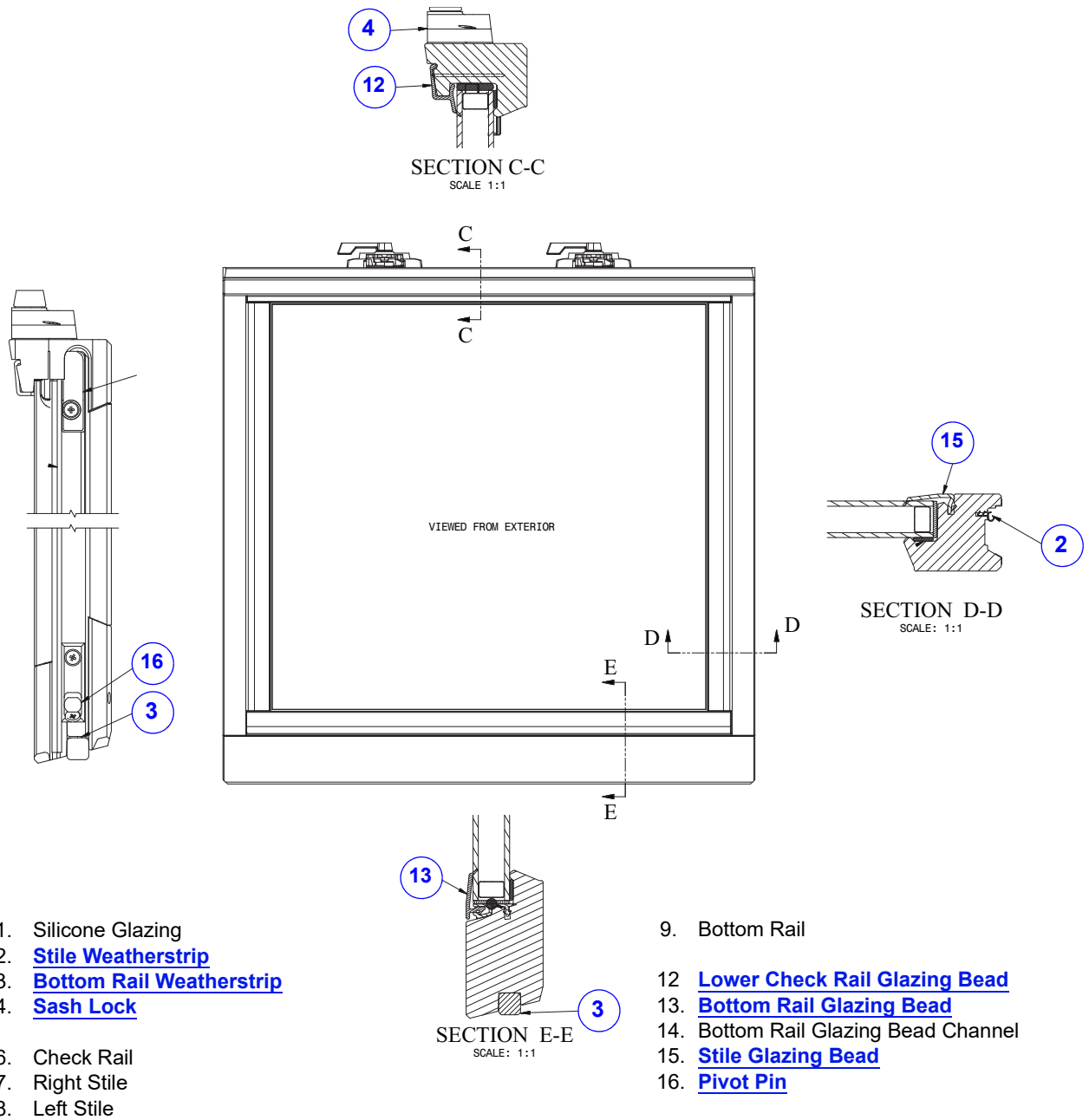
Tilt-Wash DP Upgrade (TW) Lower Sash
