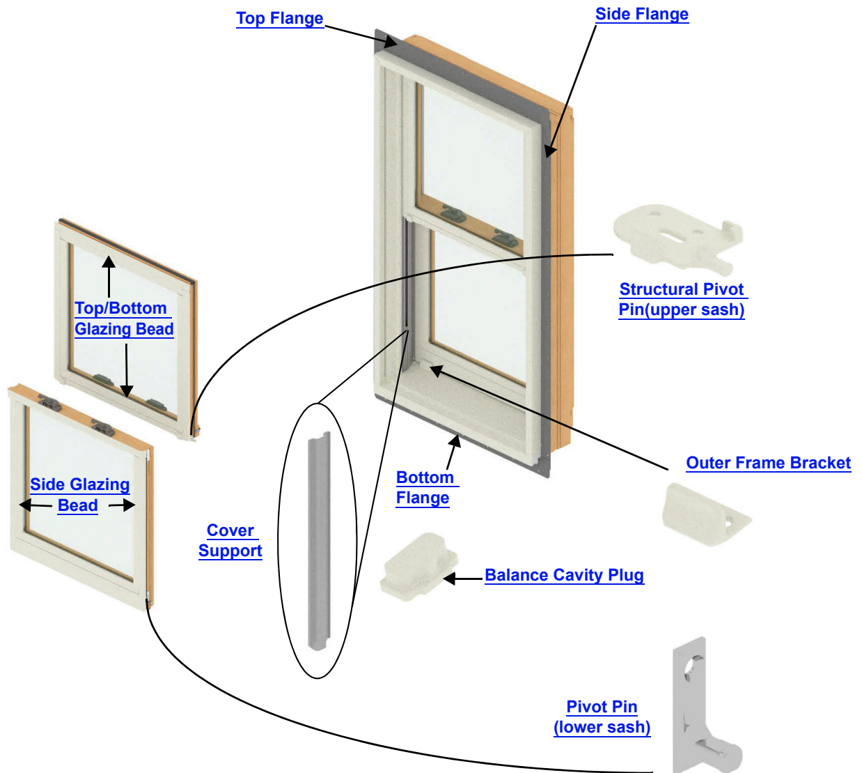
Tilt-Wash DP Upgrade Window Unit Parts
