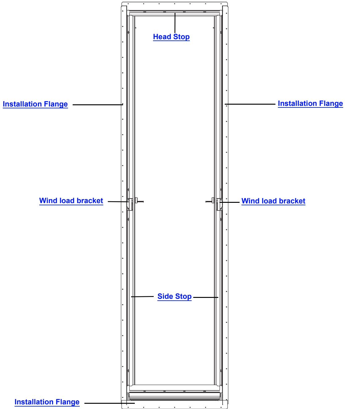
Tilt-Wash DP Upgrade Frame Assembly
