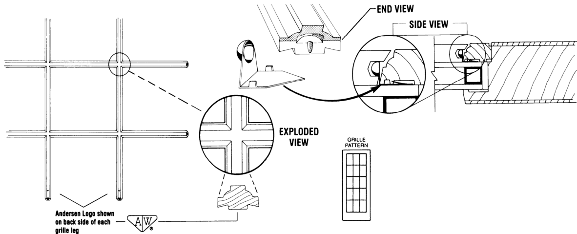
Frenchwood Gliding Door Interior Grilles / Colonial / 7/8" Wood
