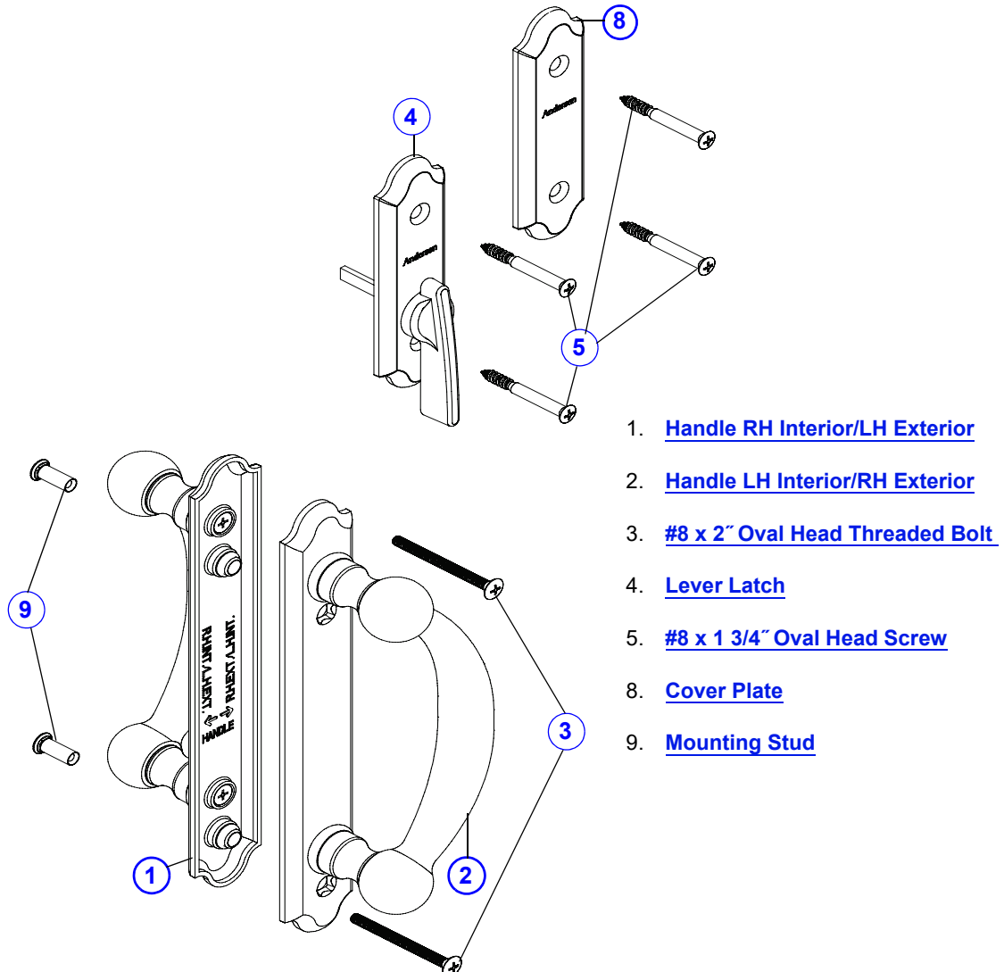
Encino® Gliding Patio Door Hardware - 2-Panel Trim Set
