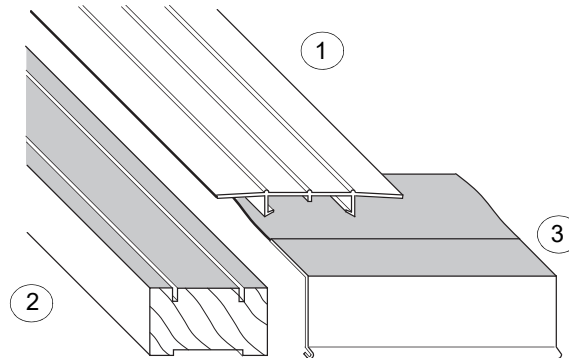
200 Series Narroline Gliding Support Mullion
