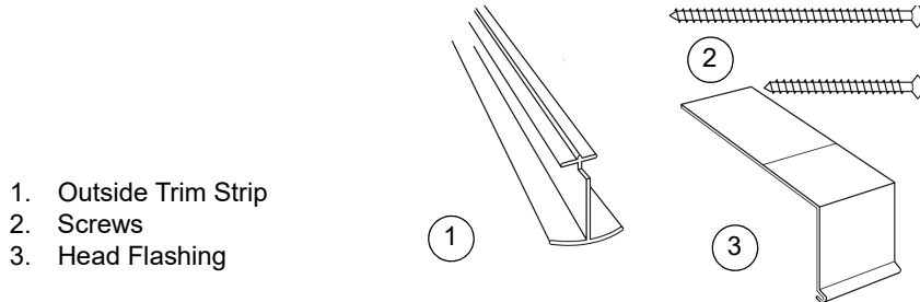
200 Series Narroline® Gliding Narrow Mullion
