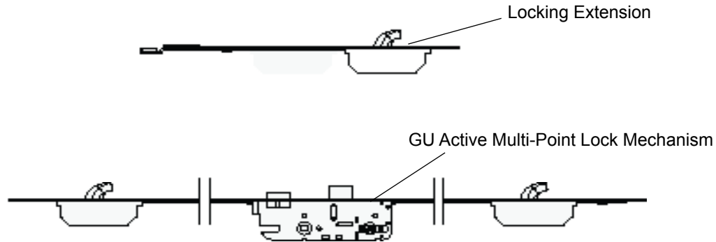
Clad Outswing Entry Doors - GU Active Lock Assembly
