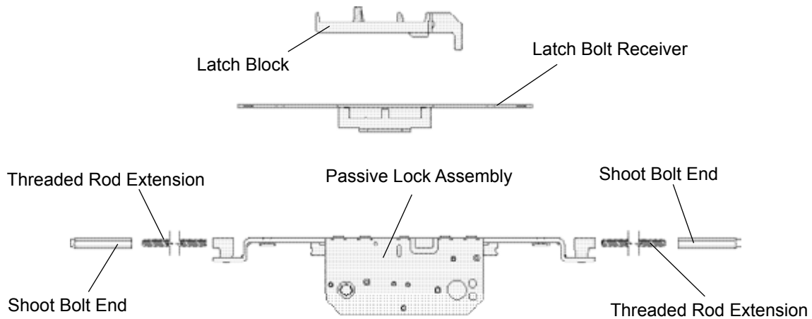
Clad Inswing Doors - AW Passive Lock Assembly
