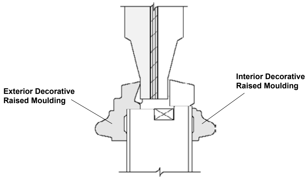
Wood Outswing Entry Doors - Decorative Raised Mouldings
