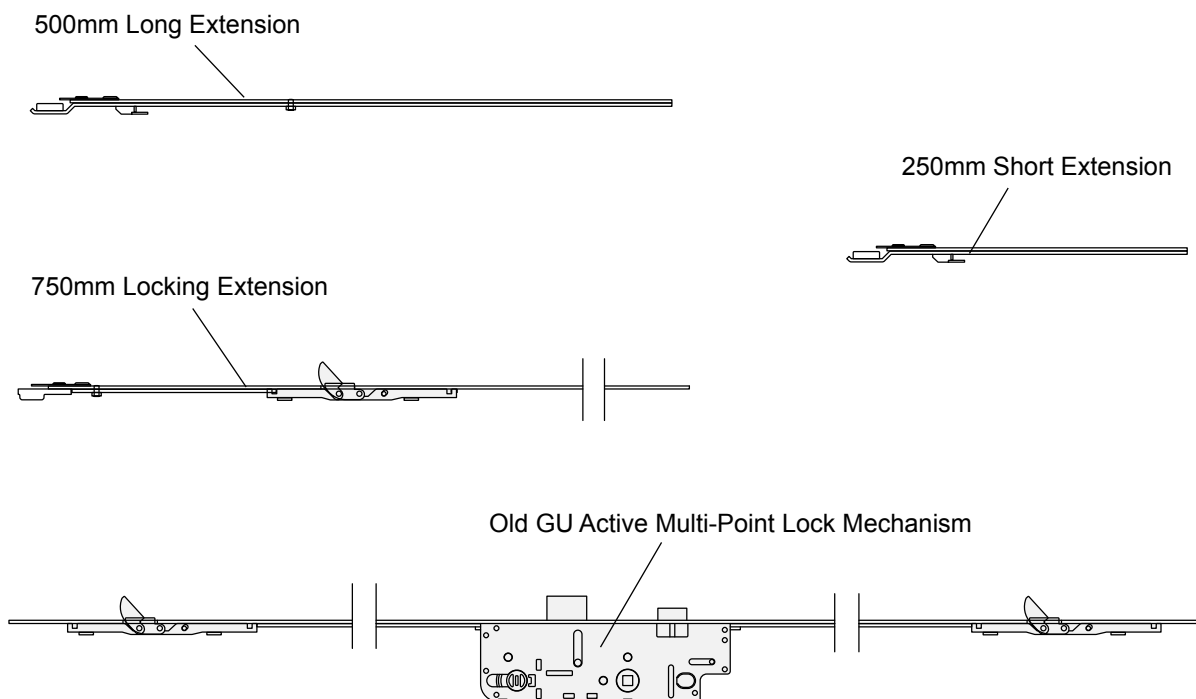
Clad Outswing Entry Doors - Old GU Active Lock Assembly
