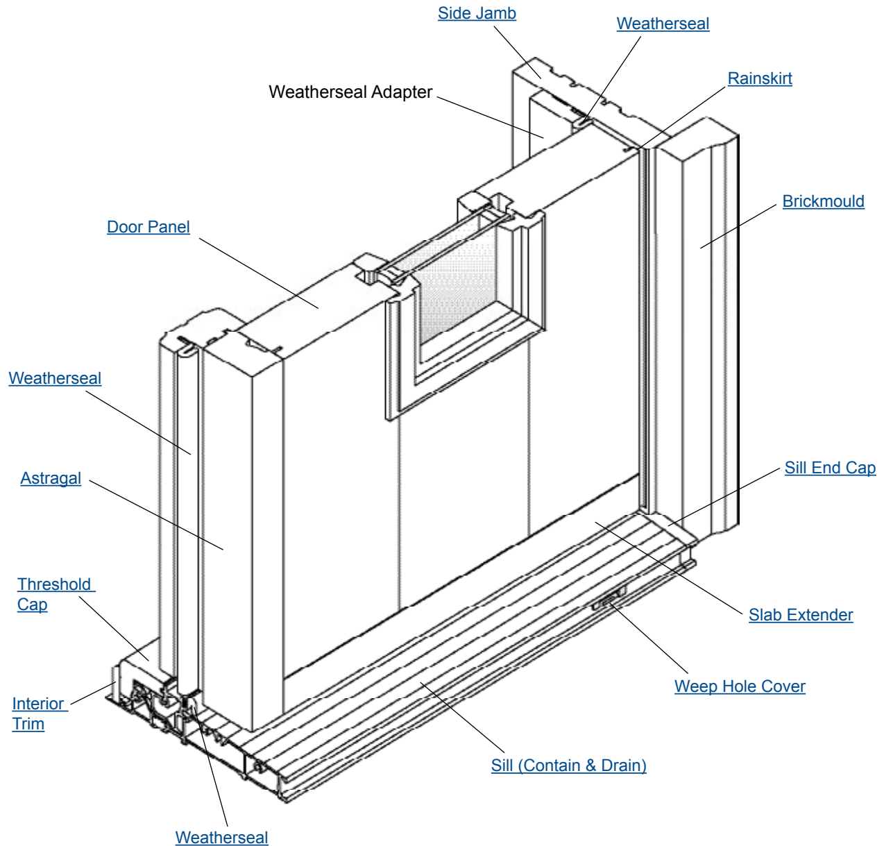
Wood Outswing Entry Doors - Passive Door
