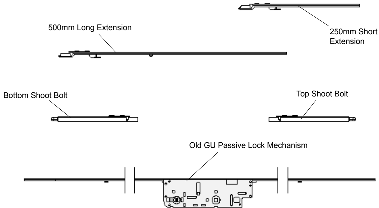
Wood Outswing Entry Doors - Old GU Passive Lock Assembly
