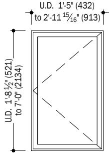
Casement
