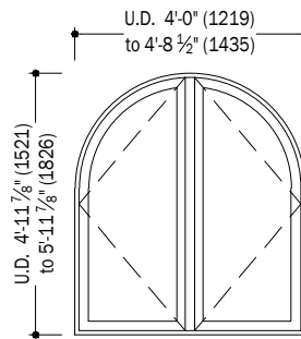
French Casement Springline
