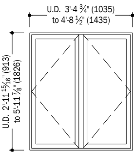
French Casement
