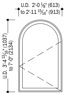
Casement Springline
