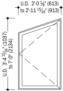
Casement Trapezoid
