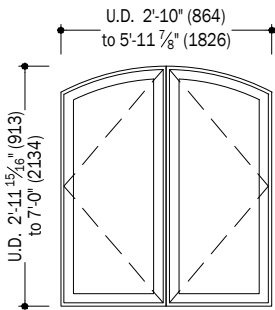
Casement Twin Archtop
