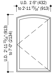
Casement Archtop
