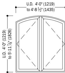
French Casement Archtop
