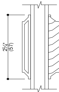
D 6 2 1/4" Simulated Divided Light Simulated check rail
