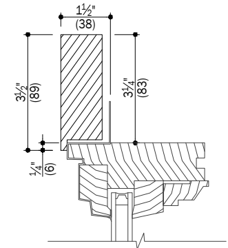
H 4 3 1/2" Flat Casing Select specialty windows are available with exterior trim. Contact your Andersen supplier for details.
