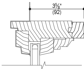
B 4 Wide Drywall Return
