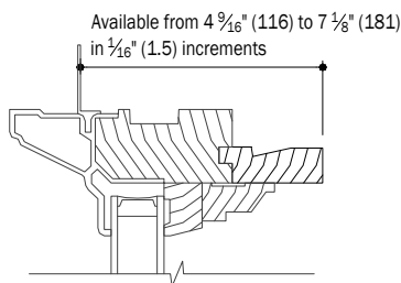
C 4 Head Fixed
