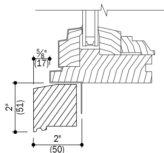
F 4 Sill Nose Select specialty windows are available with exterior trim. Contact your Andersen supplier for details.
