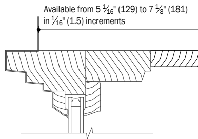
D 4 Head Fixed
