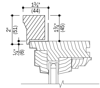
G 4 2" Brick Mould Select specialty windows are available with exterior trim. Contact your Andersen supplier for details.
