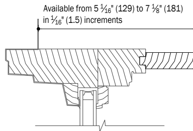
E 4 Head Fixed
