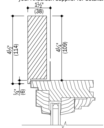
J 4 4 1/2" Flat Casing Select specialty windows are available with exterior trim. Contact your Andersen supplier for details.
